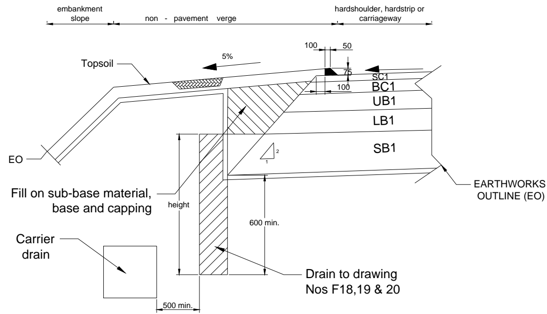
FLEXIBLE PAVEMENT
