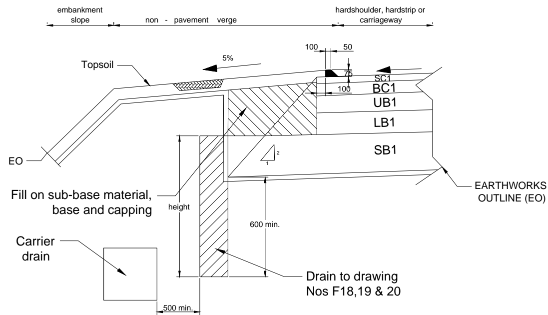
RIGID PAVEMENT
